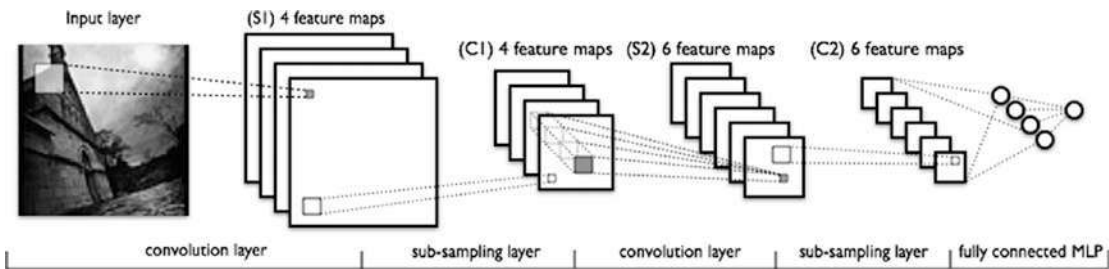
Figure 12-1. LeNet CNN model (source: deeplearning.net)
