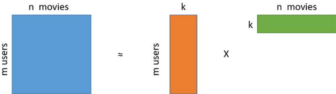
Figure 10-9. Matrix Factorization
