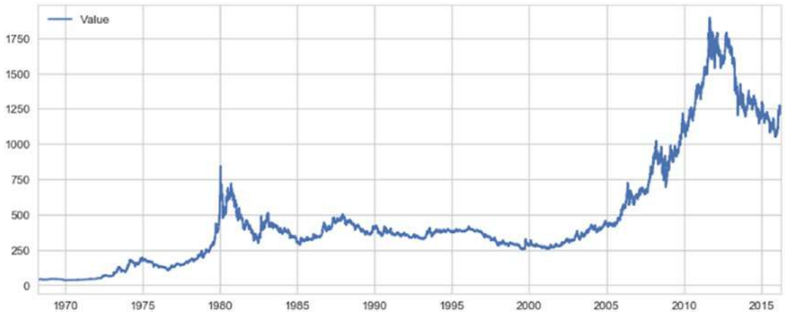
Figure 11-5. Gold prices over the years
